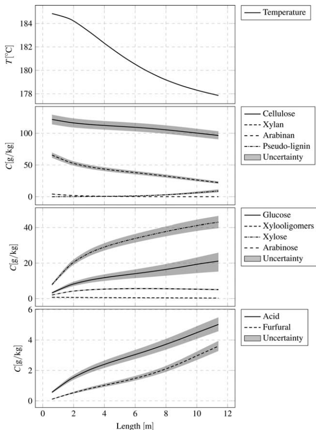
Figure 8. The top plot shows the reactor horizontal temperature gradient, which is used for calculating the reaction rates.
