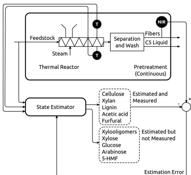
Figure 10. State estimator block diagram.
