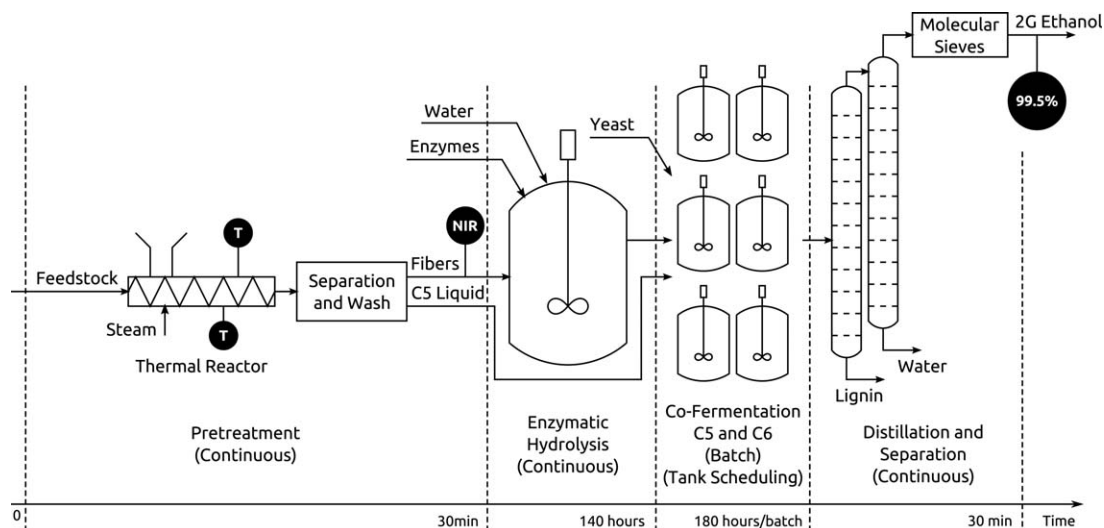
Figure 1. Process flow diagram for a second generation biorefinery: pretreatment, enzymatic hydrolysis, C5 and C6 cofermentation, and purification.
