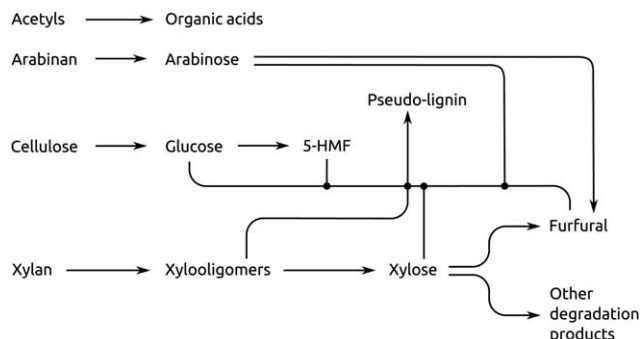
Figure 4. Hydrothermal pretreatment conversion mechanism.
