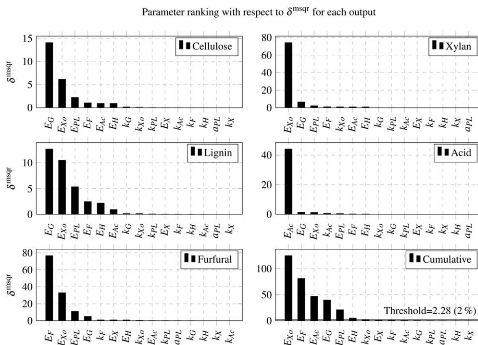
Figure 6. Sensitivity analysis by calculating the \delta^{msqr} for each output with respect to each model parameter.
