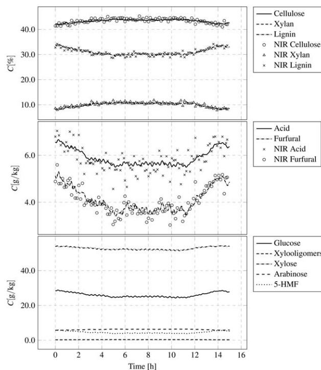
Figure 11. Pretreatment state estimator throughout 15 h of operation.
