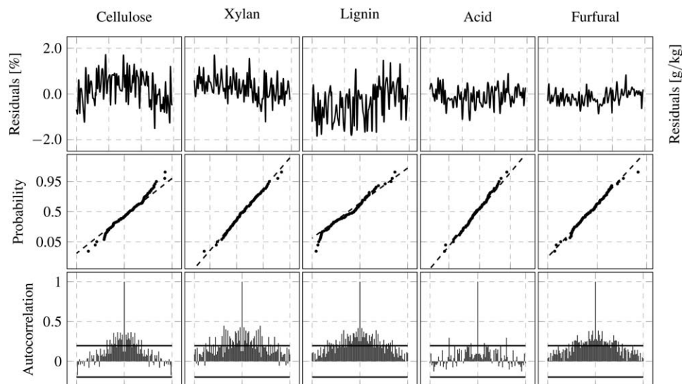
Figure 9. Residual analysis for the validation set.
